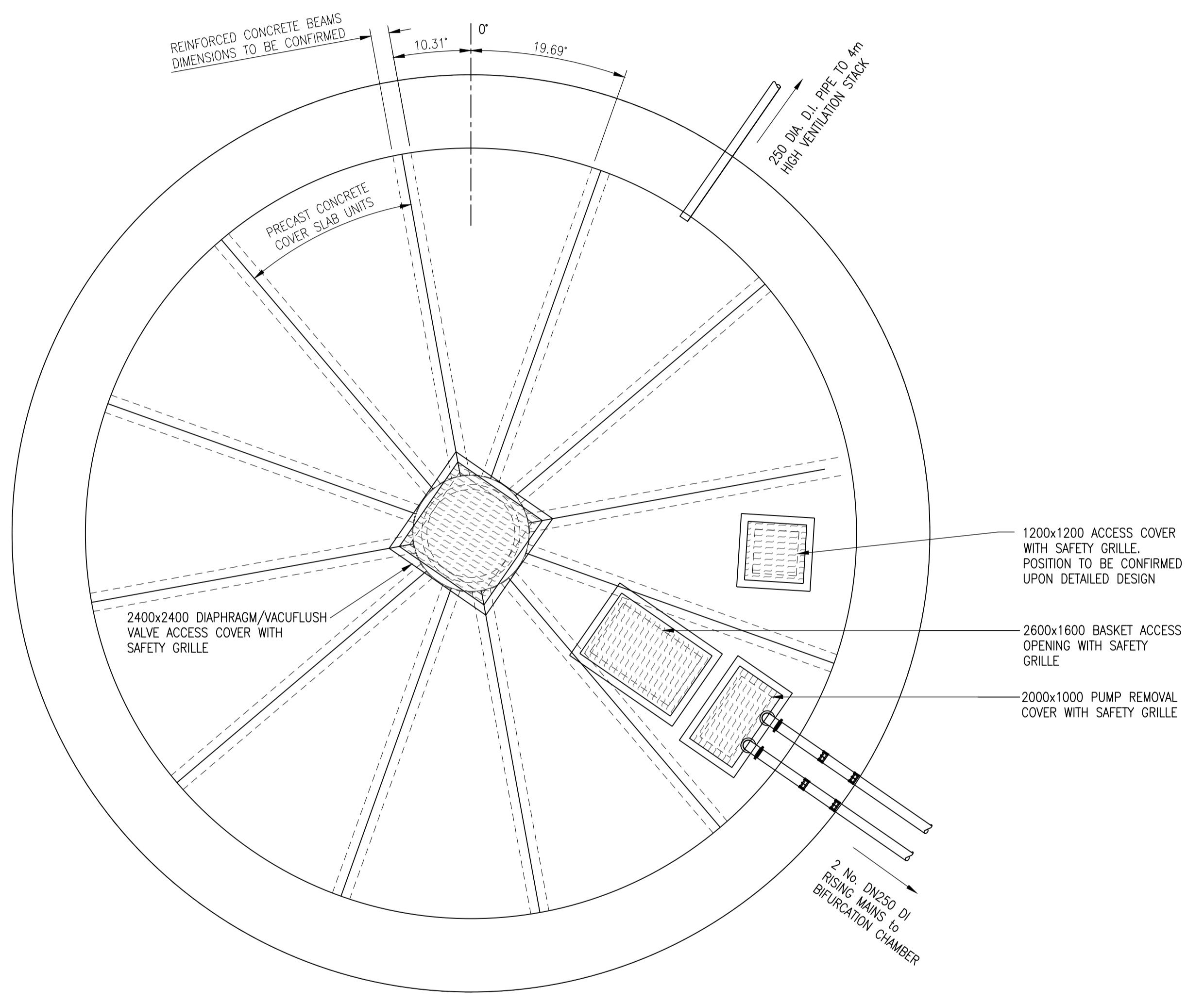
PLAN 2-2
