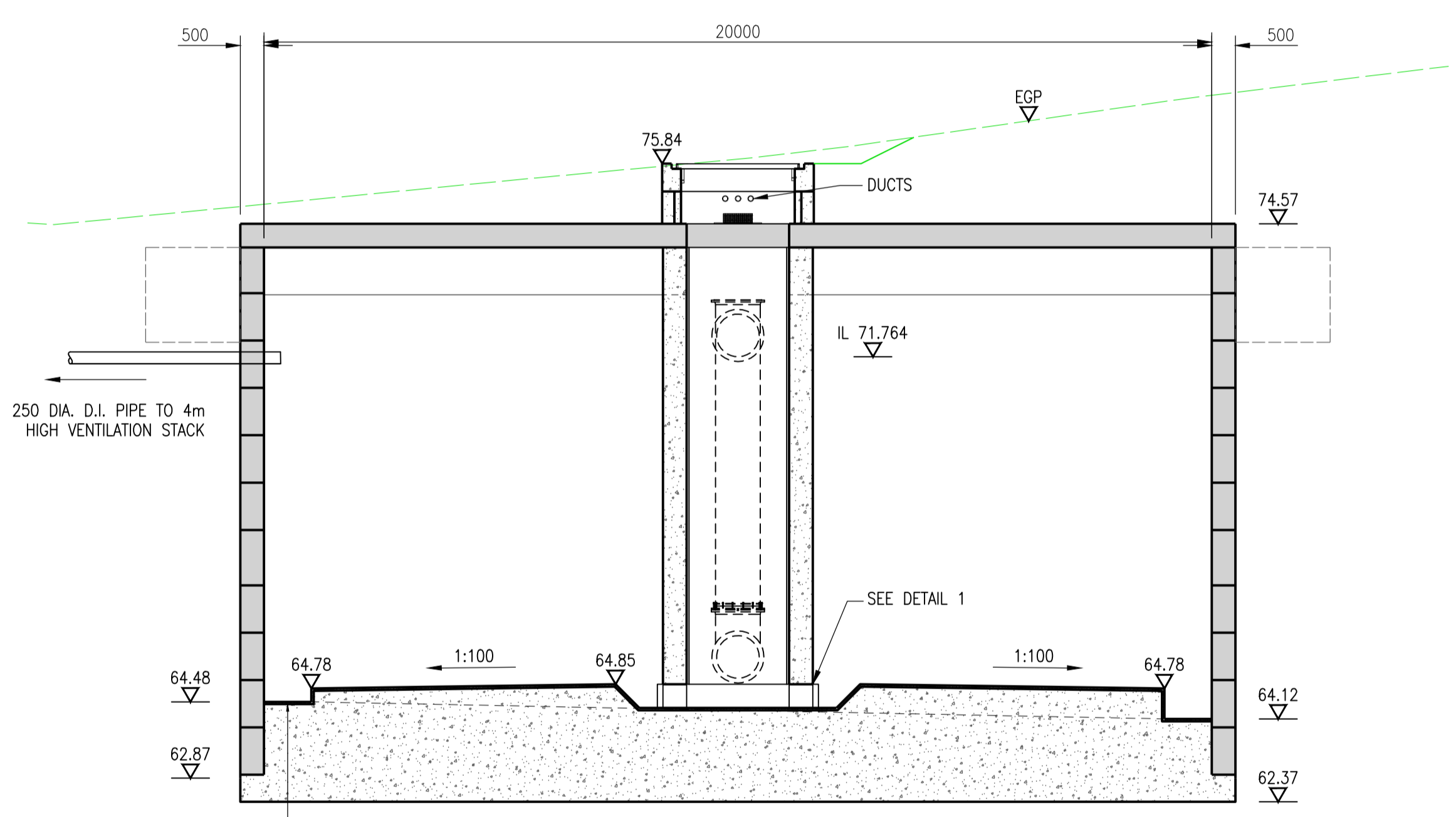
SECTION B-B
