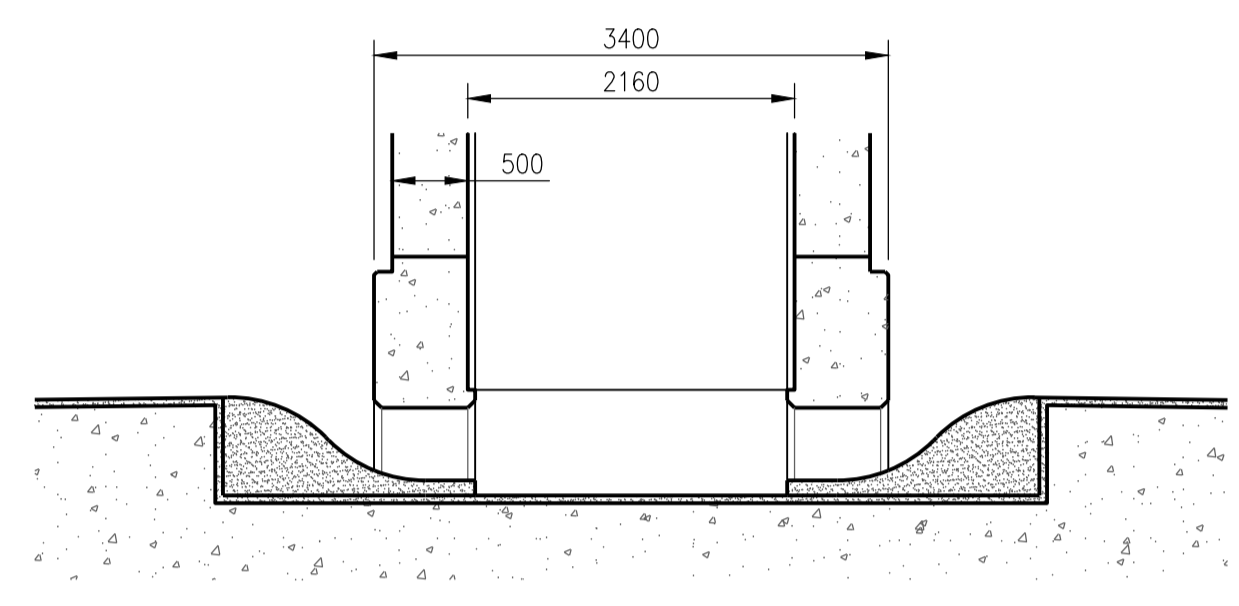
SECTIONAL ELEVATION
