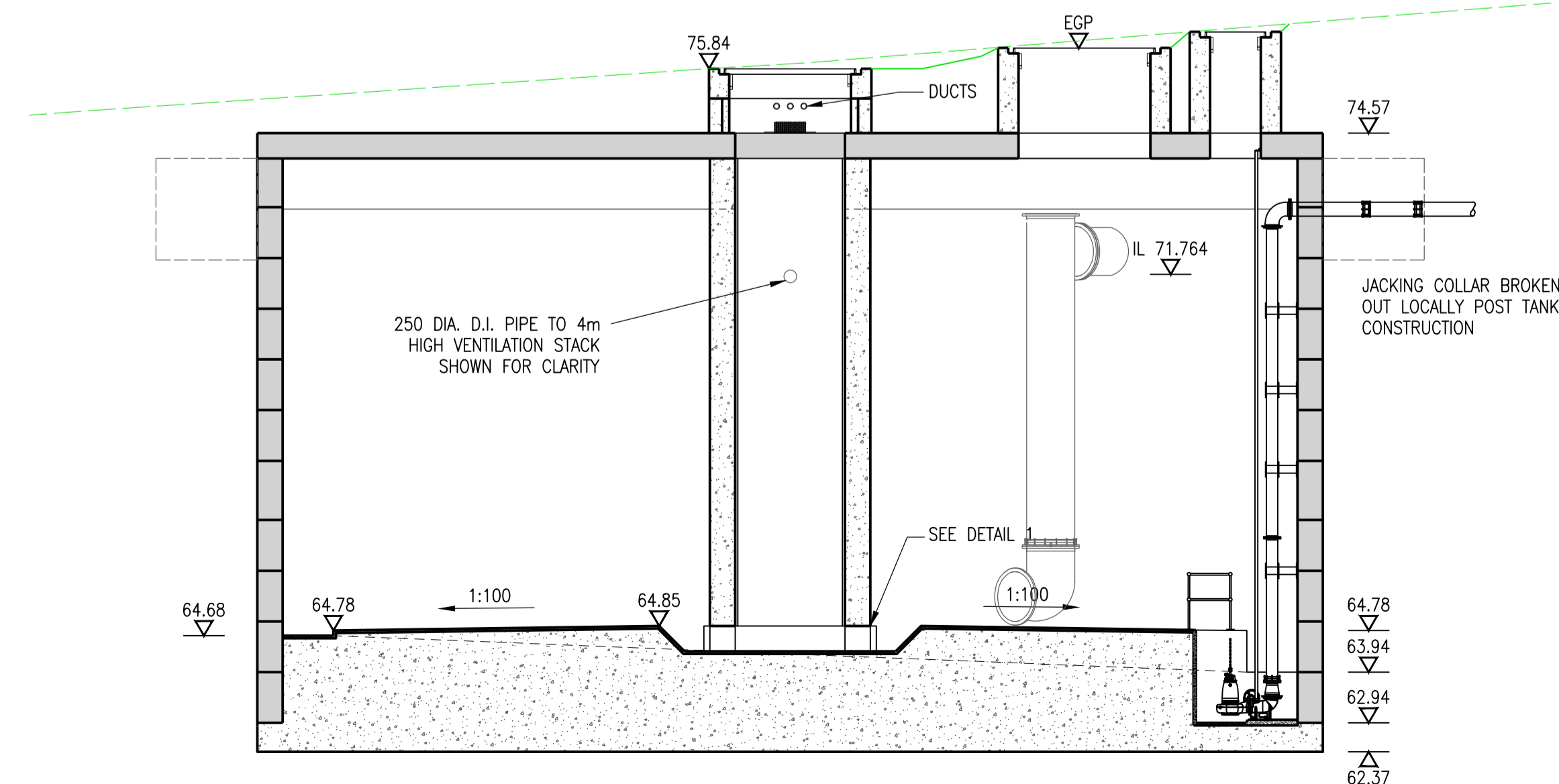
SECTION C-C
