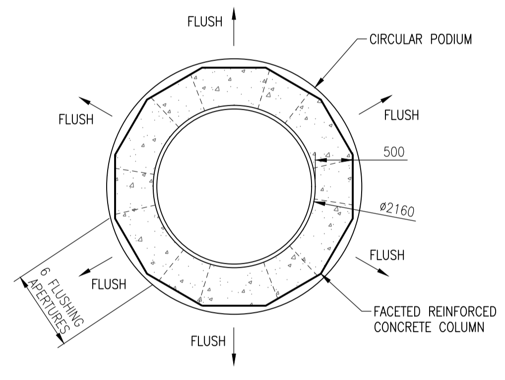
SECTIONAL PLAN DETAIL 1
